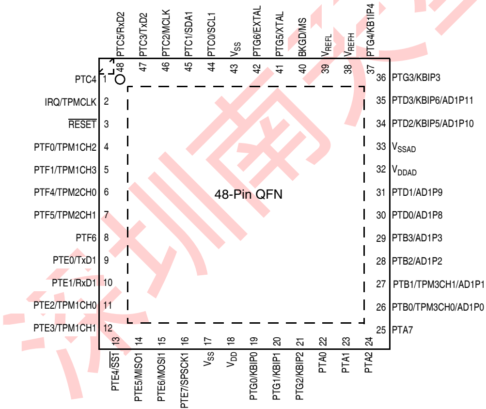
Figure 2-1. MC9S08AC16 Series in 48-Pin QFN Package
